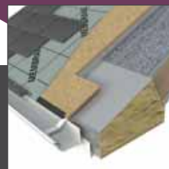
Fully insulated box beam eliminates the risk of condensation
