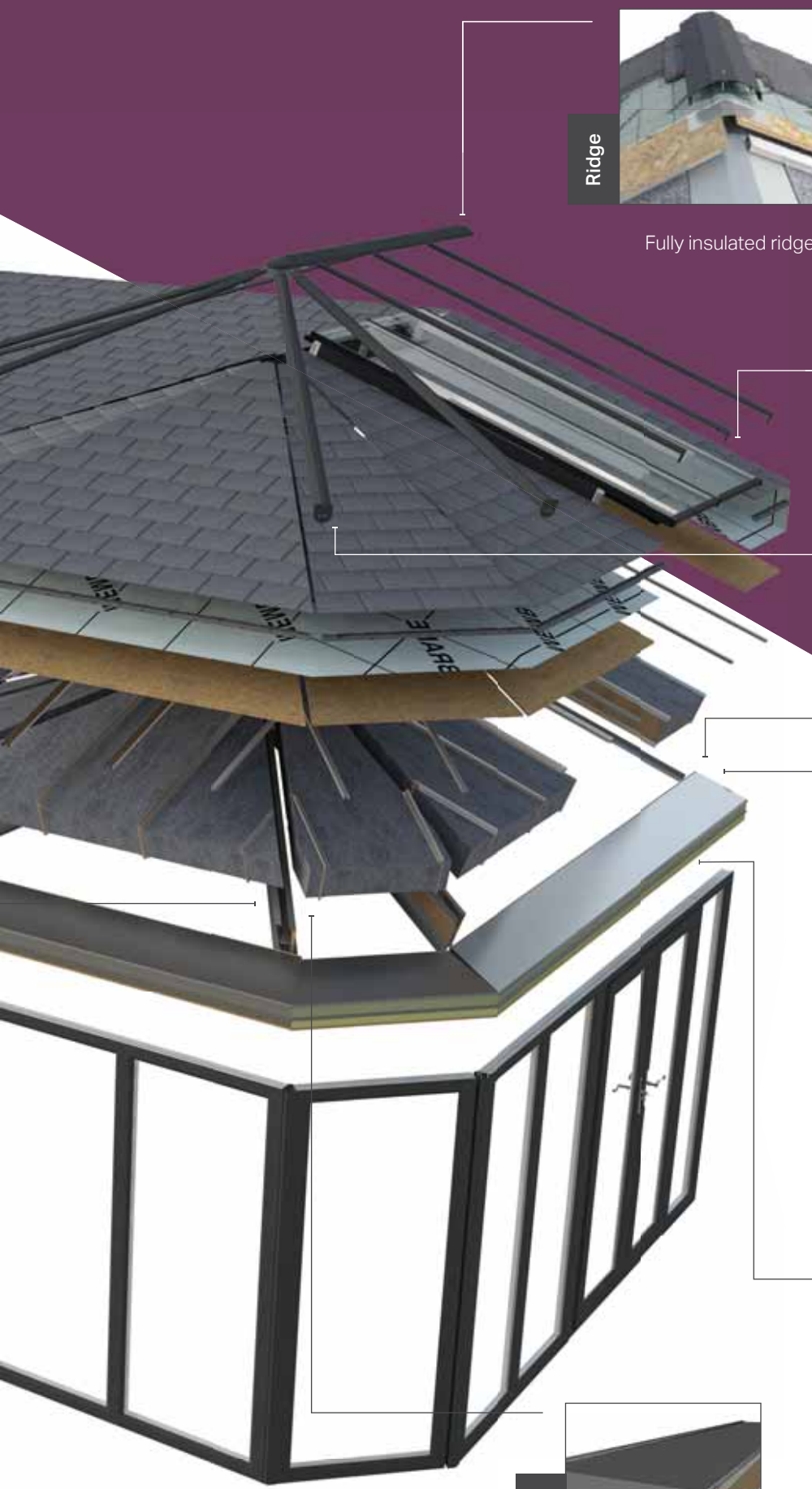
Structural insulation within the timber and steel Ultrapanel helps the roof deliver a U-Value of 0.17 (as low as 0.13 if required)
